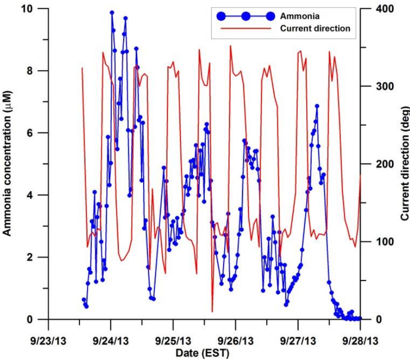
Figure 9. Ammonium concentrations are plotted with current direction.
