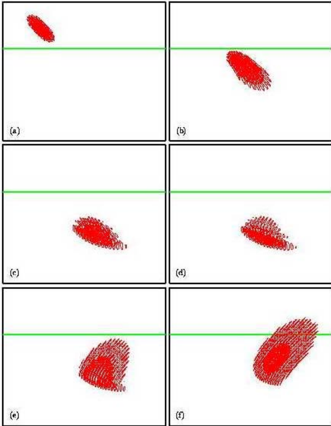
Figure 1. Contours of perturbation density showing propagation of an internal wave packet. The area shown is a vertical cross section meant to model the lower portion of the thermocline. The mean unperturbed density in this model has a constant Brunt-Vaisala frequency N above the green line. Below this line, the frequency decreases with depth. The packet propagates from the high N region downward into the region of decreasing N . On reaching a depth at which the frequency of the packet is greater than N , the packet is reflected and begins to move upward back to the region of higher N .
