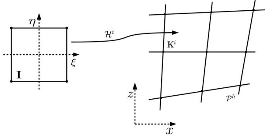
Fig. 7: Mapping from reference, (\xi, \eta) , to physical space, (x, z) . \forall K^i \in \mathcal{P}^h : K^i = \mathcal{H}^i(I) .
