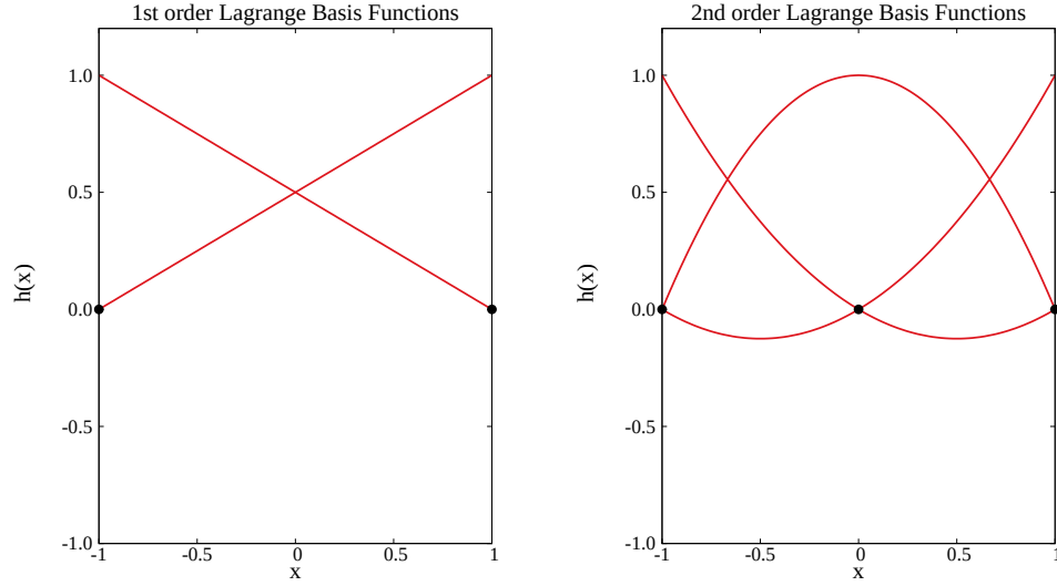
Fig. 8: Lagrange polynomials of order 1 (left) and 2 (right) along the 1D reference element \mathbf{I} = [-1, 1] . Clearly, they are equivalent for FE and SE.
