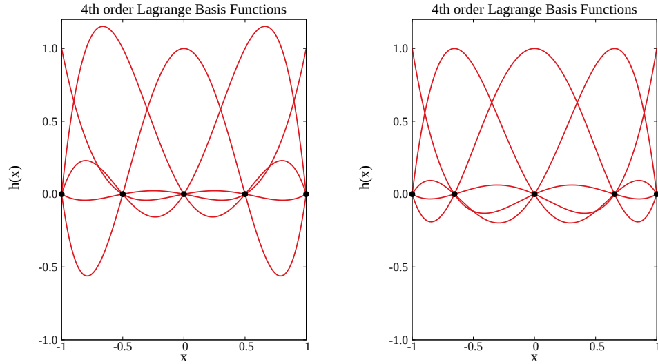
Fig. 9: Basis functions of order 4 along the 1D reference element \mathbf{I} = [-1, 1] . Left: the nodes within the element are equi-spaced as for classical high-order FE. Right: Lagrange-Legendre polynomials of order 4 whose roots are the non-equi-spaced Legendre-Gauss-Lobatto (LGL) quadrature points. Nodal SE and DG may employ LGL or LG quadrature. However, to obtain a diagonal mass matrix then LGL is the only choice for SE, while LG can still be used for DG.
