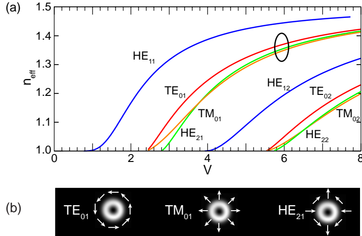
Fig. 1. (a) n_{eff} indices of several low-order modes in a nanofiber with n_{clad} = 1.5 , surrounded by vacuum ( n_{air} = 1 ). Below V \approx 3.8 , two families of modes exist. In this work, we are emphasizing the LP_{11} family (circled). By symmetry, modes in this family can interfere with the TM_{02} , TE_{02} , HE_{22} family, which may be excited through non-adiabatic processes. (b) Intensity and polarization profiles of the LP_{11} family of modes considered in this work.
