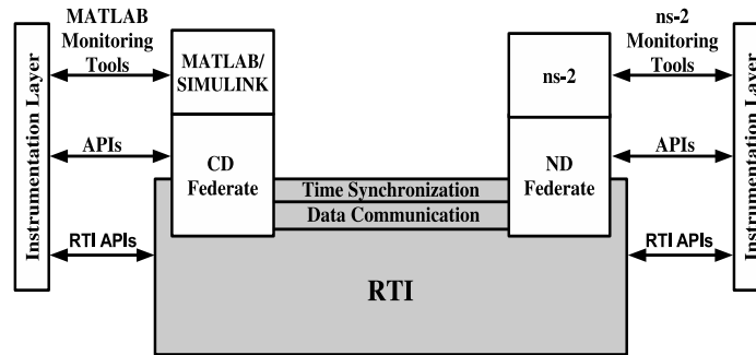
Figure 55: Run-Time Components
