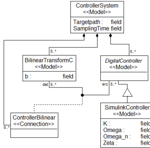
Figure 17: ControllerSystem Sub-Language (For Non-linear Plant)
