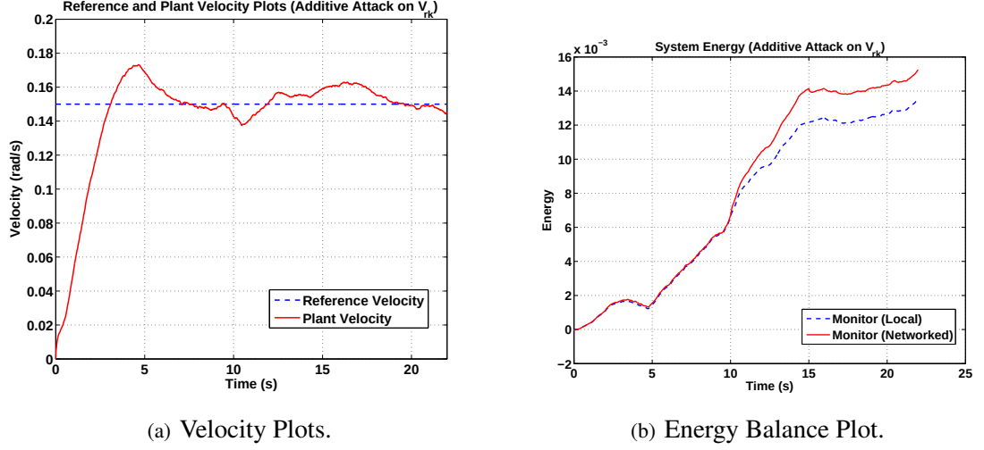
Figure 80: Experimental Results - Additive Attack on V_{rk} .
