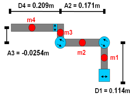
Figure 24: CrustCrawler Model
