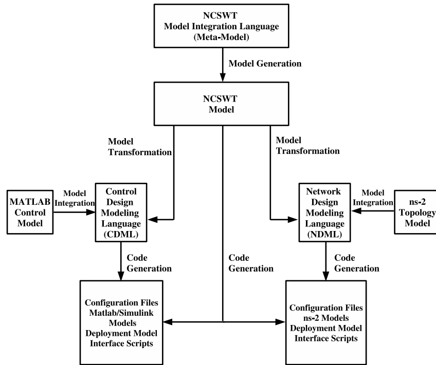
Figure 46: Model-Based Design Architecture for NCSWT
