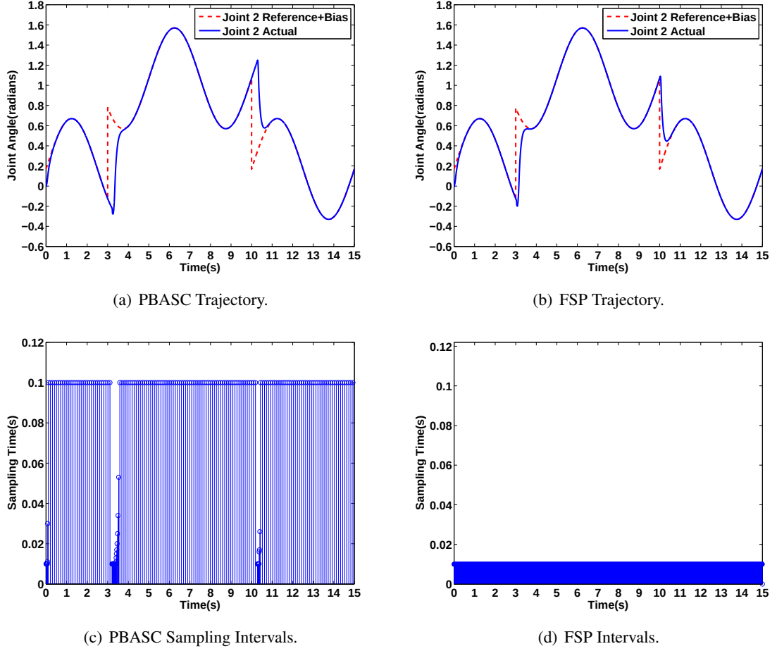
Figure 37: Simulation Results - PBASC Approach vs. FSP Approach in Nominal Case.
