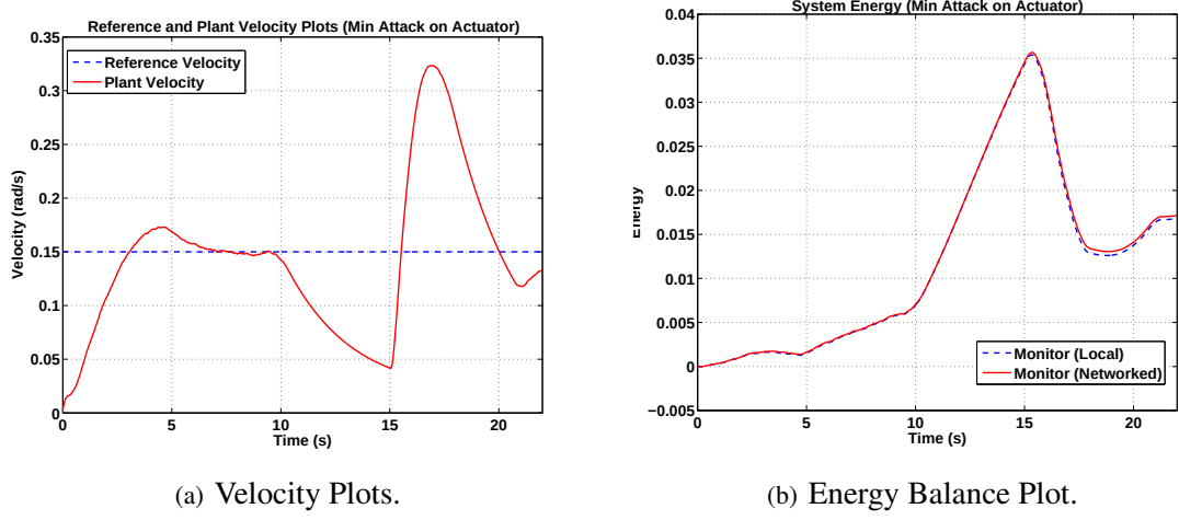
Figure 81: Experimental Results - Min Attack on Actuator, u_k .
