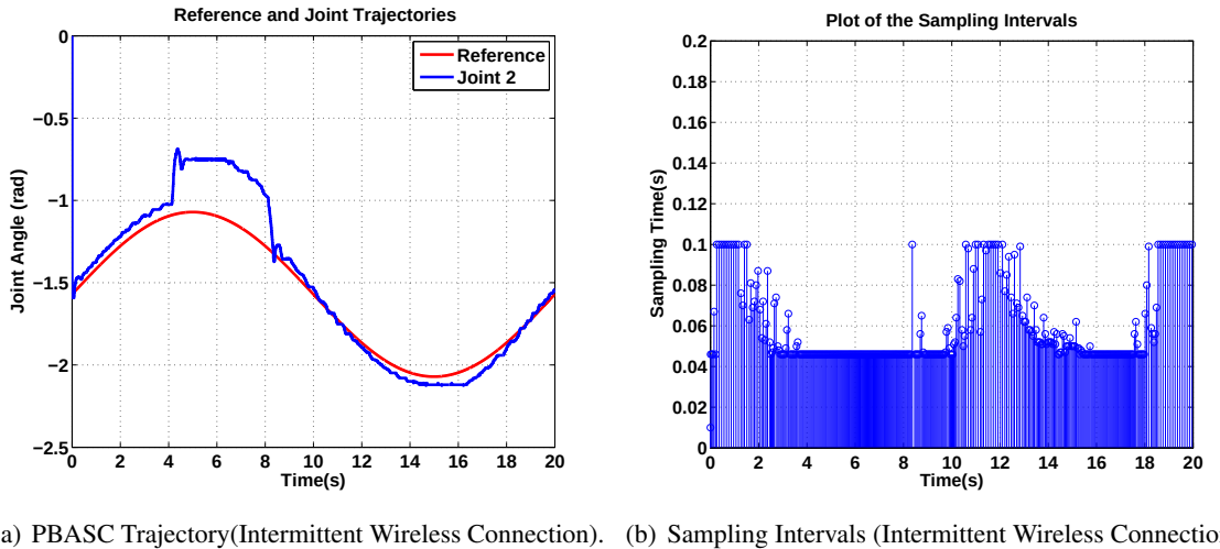
Figure 43: Experimental Results - PBASC Approach with Intermittent Wireless Connection.
