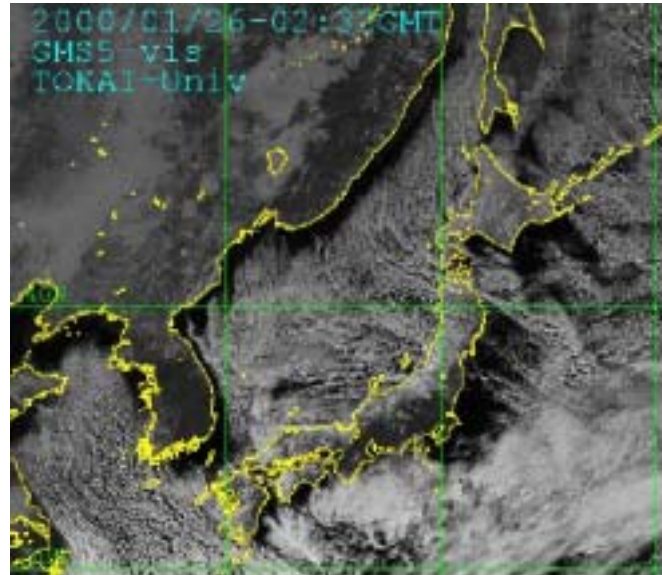
Figure 2. Marine cloud sheet over the JES during a cold-air outbreak on January 26, 2000.
