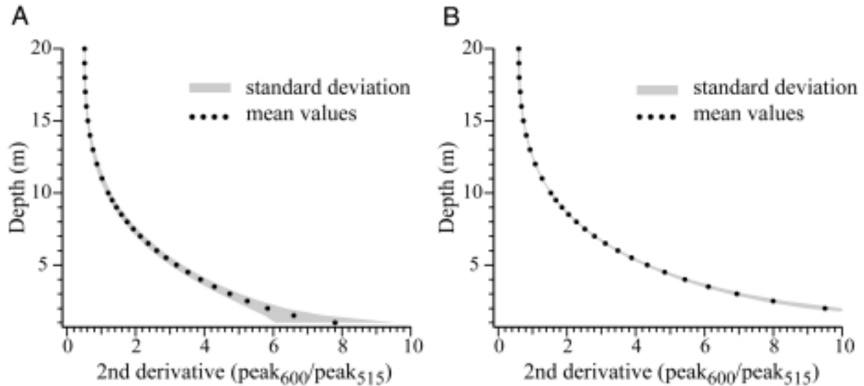
Figure 3. Mean of 2 nd derivative peak ratio (Peak 600 /Peak 515 ) versus depth for spectral library. A: sediment and seagrass B: pavement/coral
