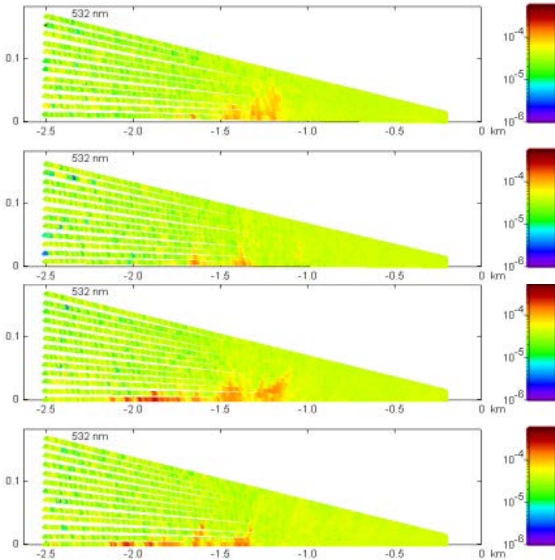
Figure 2: Vertical lidar scan of aerosol extinction taken 48°E off Bellows Beach on 3/27/01 at 09:40 HST. The wind direction is 78°E and the wind speed 7.7 m/s.
