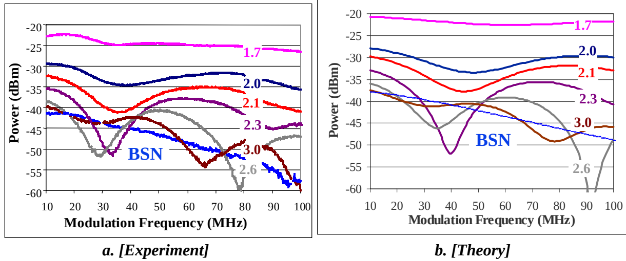
Figure 2. Experimental (a) and theoretical (b) results obtained with the parameters listed in Table 2. The power of the target and backscatter (BSN) return signals are plotted as a function of modulation frequency for several depths
