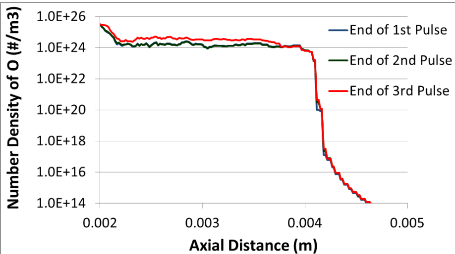
O radical density
