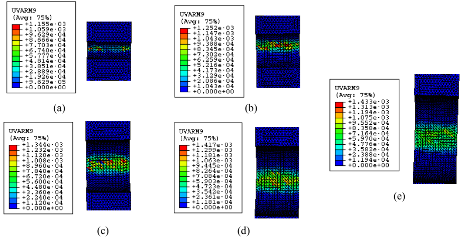
Fig. 1: Plastic strain distributions within the notch root region of a double-edge notched plate (at the same strain amplitude of \epsilon_y = 0.027\% and strain ratio R_\epsilon = -1 ) for various notch root radii \rho considered (a) 200\ \mu\text{m} (b) 400\ \mu\text{m} (c) 600\ \mu\text{m} (d) 800\ \mu\text{m} (e) 1000\ \mu\text{m} .
