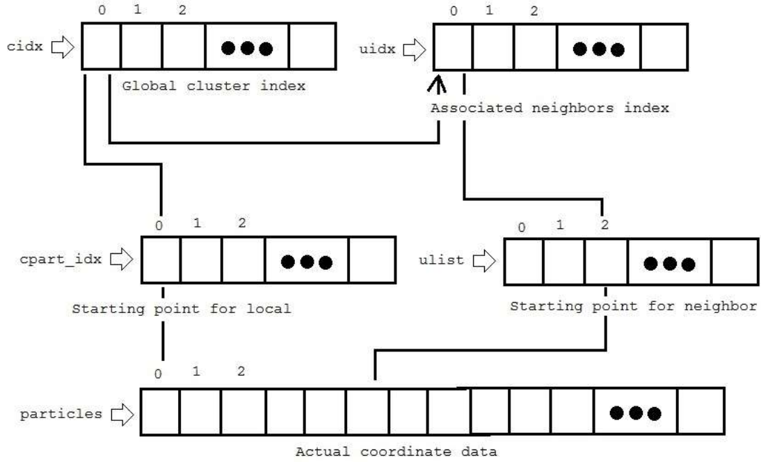
Fig. 3 P2P data and indirection pointers
