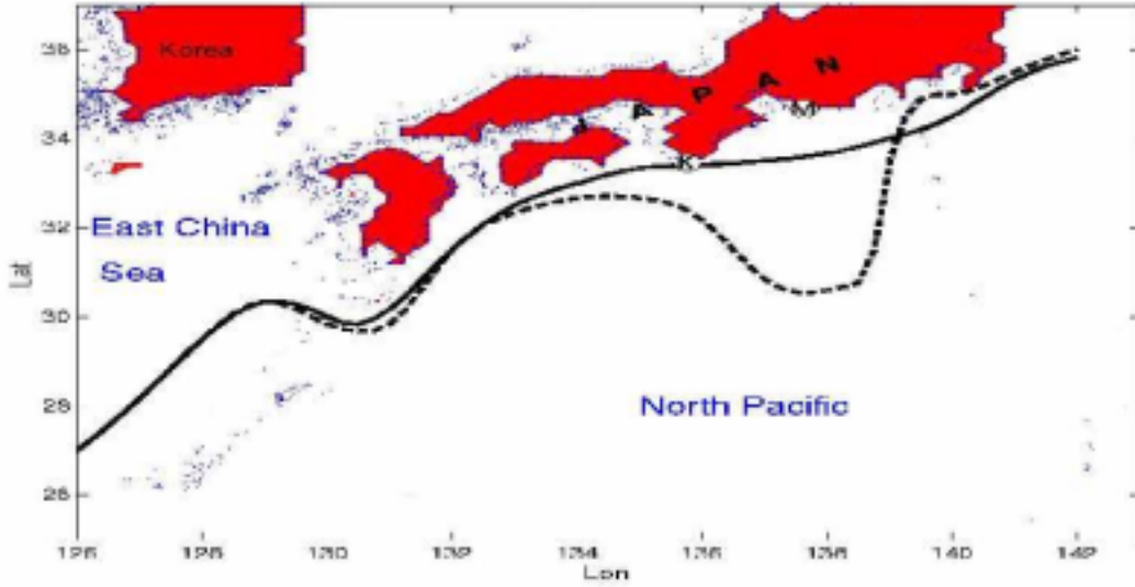
Figure 1. Typical paths of the Kuroshio with tide gauge locations shown. “K” denotes Kushimoto, “M” denotes Maisaka.
