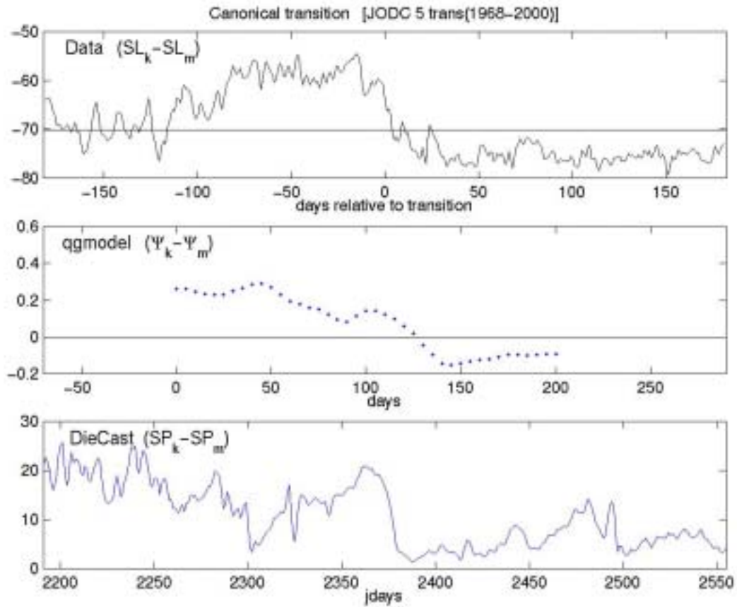
Figure 2. Evolution of sea level difference between Kushimoto and Maisaka as indicator for transition from non-large meander to large meander state. Top: observed sea level difference; center: Transport streamfunction difference in quasigeostrophic model corresponding to sea level difference; bottom: DieCast simulation of sea level difference.
