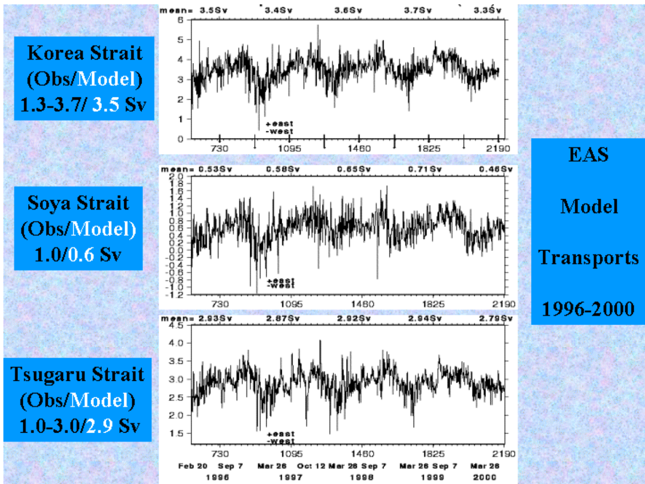
Figure 1. The EAS-year model time series of transport through the Korea, Soya and Tsugaru Straits. The mean transport for these five years, compared to observations, shows that the modeled transport fits within the limits of the observed transports.
