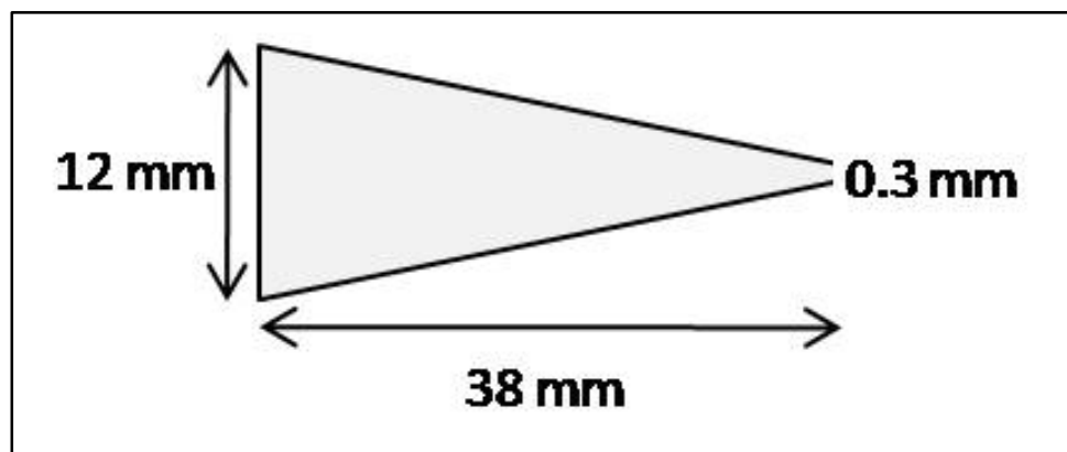
Figure 2. Near-Field Aperture Horn
