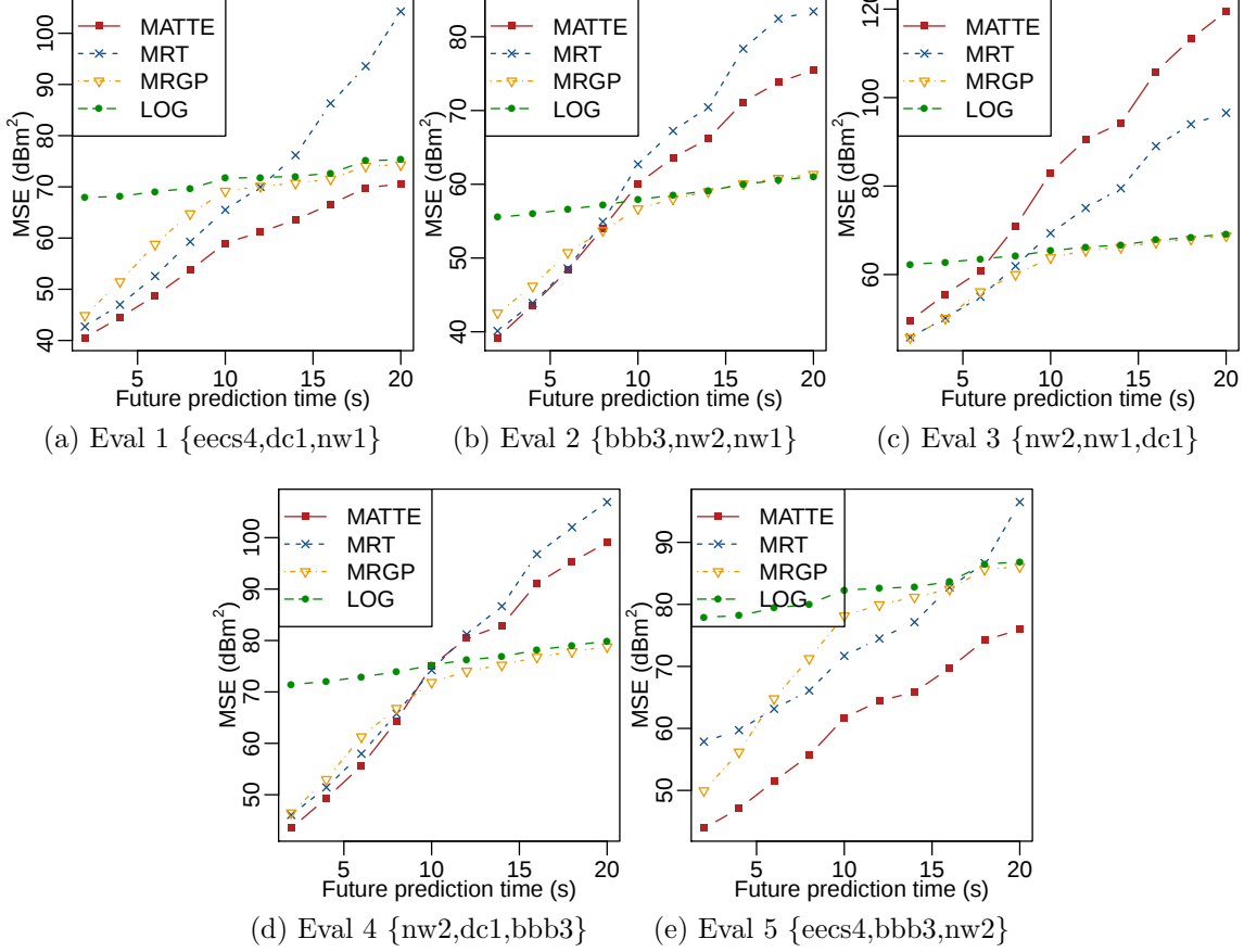
Figure 3.4: Evaluation of signal-strength prediction accuracy. MSE is shown for each method on one of the five testing datasets. Error bars are bounded by 0.8 \text{ dBm}^2 and are omitted for clarity. Our proposed method, MATTE, is compared to extensions of previous methods MRGP and MRT. Our method generally performs better for near-term predictions where the robots’ sensor data provides an informative prior. Poor performance of MATTE in evaluation 3 is attributable to the randomly generated training set which contains only indoor datasets, while the testing set contains both indoor and outdoor sets.
