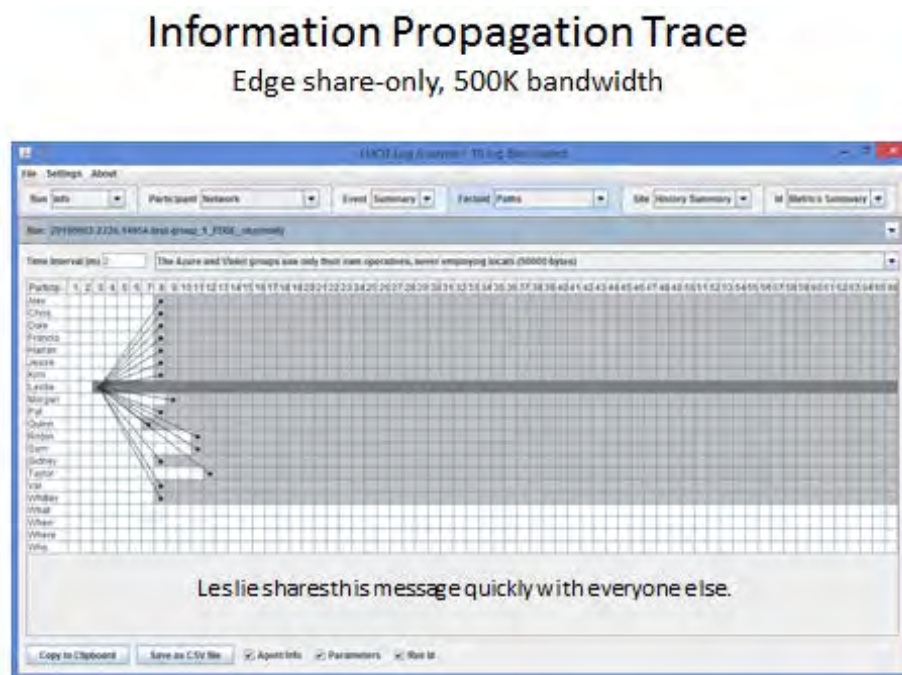
Fig. 4 Information propagation - high bandwidth
