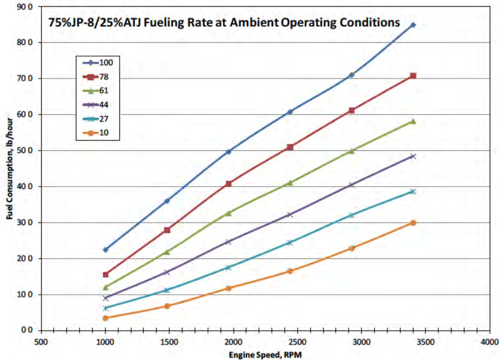
Figure 4. Fueling Rate with 75%JP-8/25%ATJ at Ambient Operating Conditions
