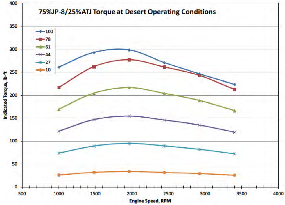
Figure 9. Indicated Torque with 75%JP-8/25%ATJ at Desert Operating Conditions
