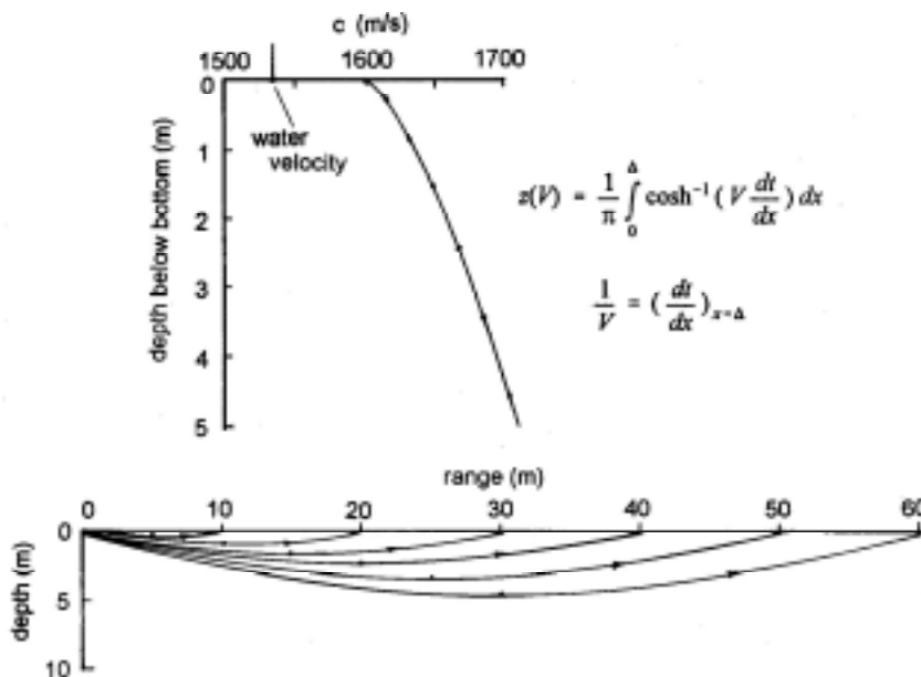
P-wave velocity versus depth obtained by Weichert, Herglotz, Bateman analysis of first arrivals and wave trajectories corresponding to different ranges
