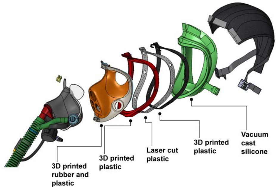
Figure 3: Aspects of the Army's Joint Service Aircrew Mask Prototyped Using Additive Manufacturing
