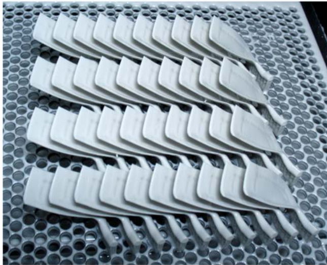
Figure 11: Defense Logistics Agency Casting Cores for Engine Airfoils (Blades and Vanes) Additively Manufactured
