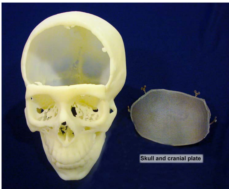
Figure 12: Walter Reed National Military Medical Center Cranial Implant Additively Manufactured
