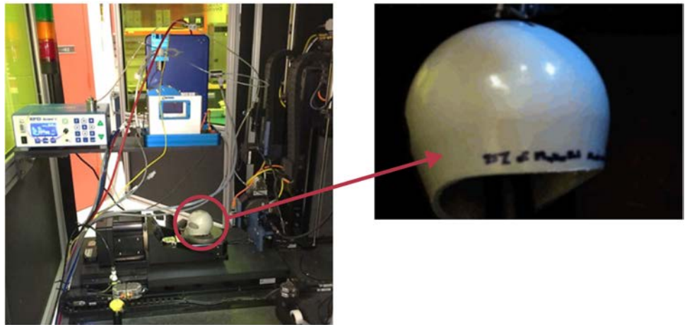
Figure 10: Air Force Is Researching How to Additively Manufacture and Embed Antennas within Helmets
