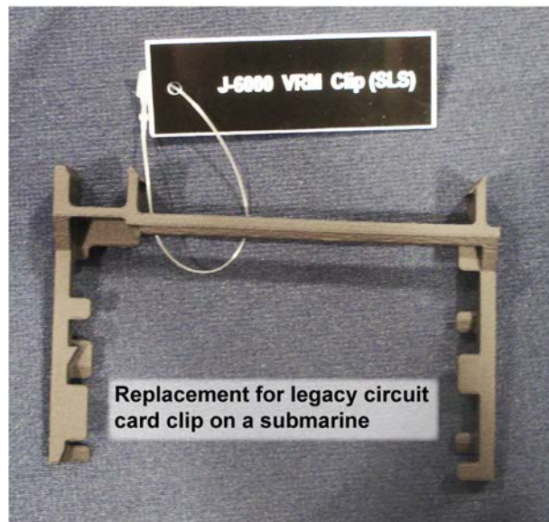
Figure 8: Navy Replacement Part for Legacy Circuit Card Clip Additively Manufactured
