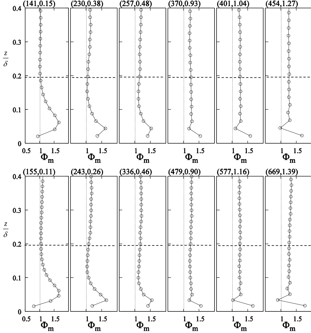
FIG. 10. Change of structure of \Phi_m(z) as the LES move towards and into the HAZ. Refer to Fig. 8 for the locations of the individual simulations on the \Re - \text{Re}_{LES} parameter space; \Re and \text{Re}_{LES} progressively increase in each panel from left to right. Top panel: LES with N_z = 96 . Bottom panel: LES with N_z = 128 . \text{Re}_{LES} and \Re are given on top of each figure, as (\text{Re}_{LES}, \Re) . \kappa = 0.4 is assumed in forming \Phi_m . \delta is defined as the height where \Phi_m = 0 . The horizontal dashed lines indicate roughly the upper-most margin of the surface layer.
