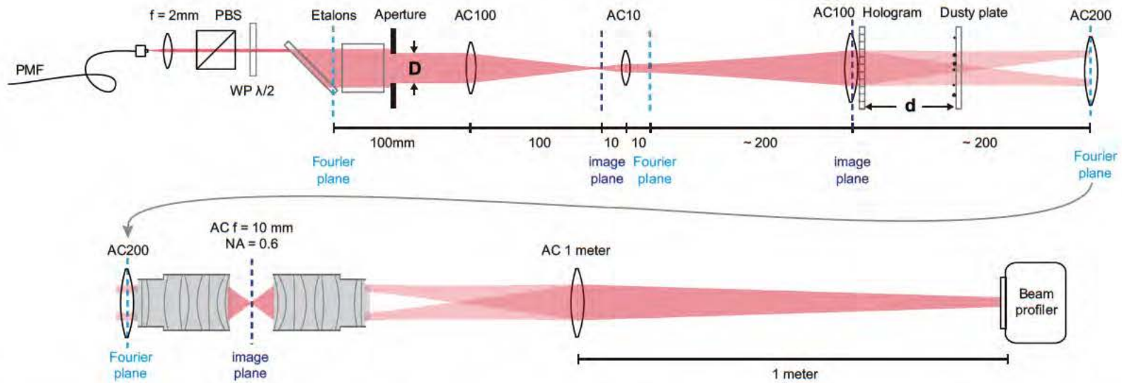
Figure 4.6: The setup used to test the performance of spatially incoherence sources. The degree of incoherence can be varied by the Fourier plane aperture D . The dusty plate at distance d from the hologram can be moved anywhere between the image plane and the Fourier plane to study the resulting disorder.
