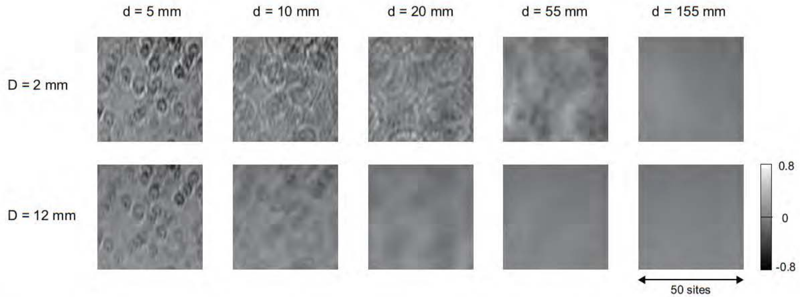
Figure 4.7: Images from the test setup illustrated in Figure 4.6, showing disordered potential caused by dust particles placed in various positions between the image plane and the Fourier plane. Top row for spatially coherent source, and bottom row for spatially incoherent source. A constant DC offset has been removed from the images to show the disorder. The color bar is in units of the DC offset.
