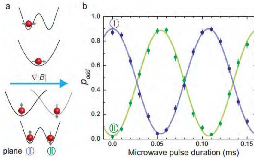
Figure 7.9: Spin-resolved readout. (a) Procedure for mapping the hyperfine spin onto different axial planes: After reducing the tunnel barrier in a double-well with an arbitrary spin in plane I to zero, a B-field gradient separates the |\uparrow\rangle and |\downarrow\rangle components into different axial planes. The two hyperfine states will appear in different planes in imaging. (b) A resonant microwave pulse is applied to a n = 1 Mott insulator in state |\uparrow\rangle in plane I. The sinusoidal variation in hyperfine spin is mapped onto occupation in plane I (blue) and plane II (green). Solid lines are fits with sine functions.
