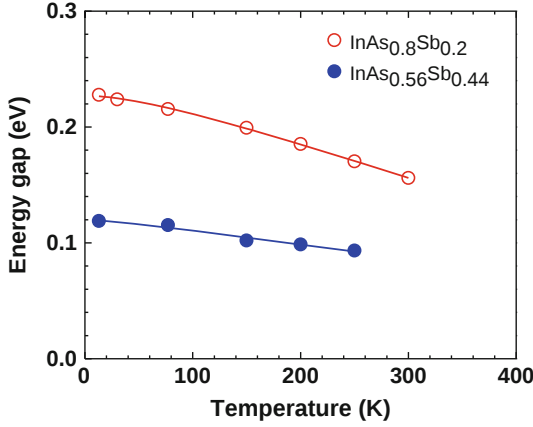
Fig. 8. Temperature dependences of the energy gaps of bulk InAs 0.8 Sb 0.2 (a) and InAs 0.56 Sb 0.44 (b). The fits were obtained using the following Varshni parameters: E_{g0} = 0.226 eV, \alpha = 3.2 meV/K, and b = 100.4 K for InAs 0.8 Sb 0.2 ; E_{g0} = 0.119 eV, \alpha = 1.2 meV/K, and b = 33.3 K for InAs 0.56 Sb 0.44 .
