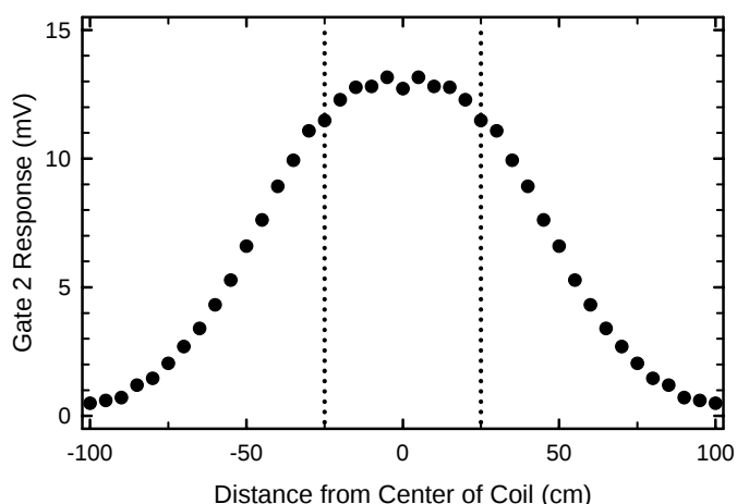
Figure 2-5. Anomaly amplitude as a function of cross-track position for a 37-mm projectile horizontal, along-track 50 cm below the coil of an EM61-MK2. The coil is 1 m wide. The vertical dotted lines at \pm 25 cm represent the maximum offset of an object passing under the coil at 0.5-m line spacing.
