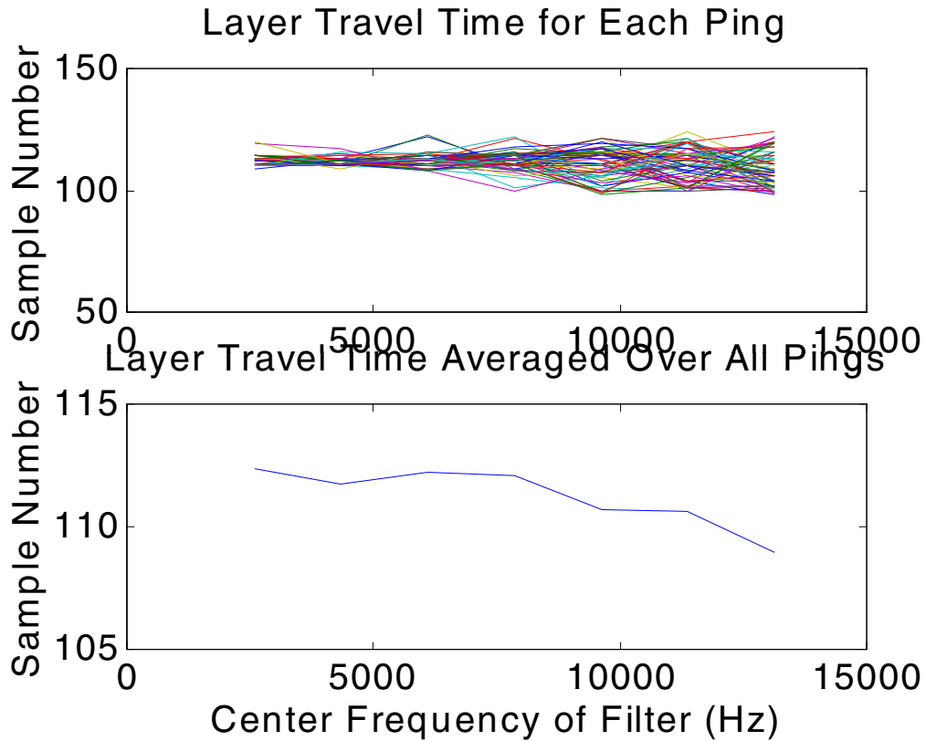
Figure 1 a) Two way echo travel time (in samples) as a function of frequency for 50 transmissions. The noisy measurements must be averaged to obtain an accurate estimate of phase dispersion. b) The graph of mean two way echo travel time as a function of frequency shows that travel time decreases with increasing frequency, or equivalently, sound speed increases with frequency.
