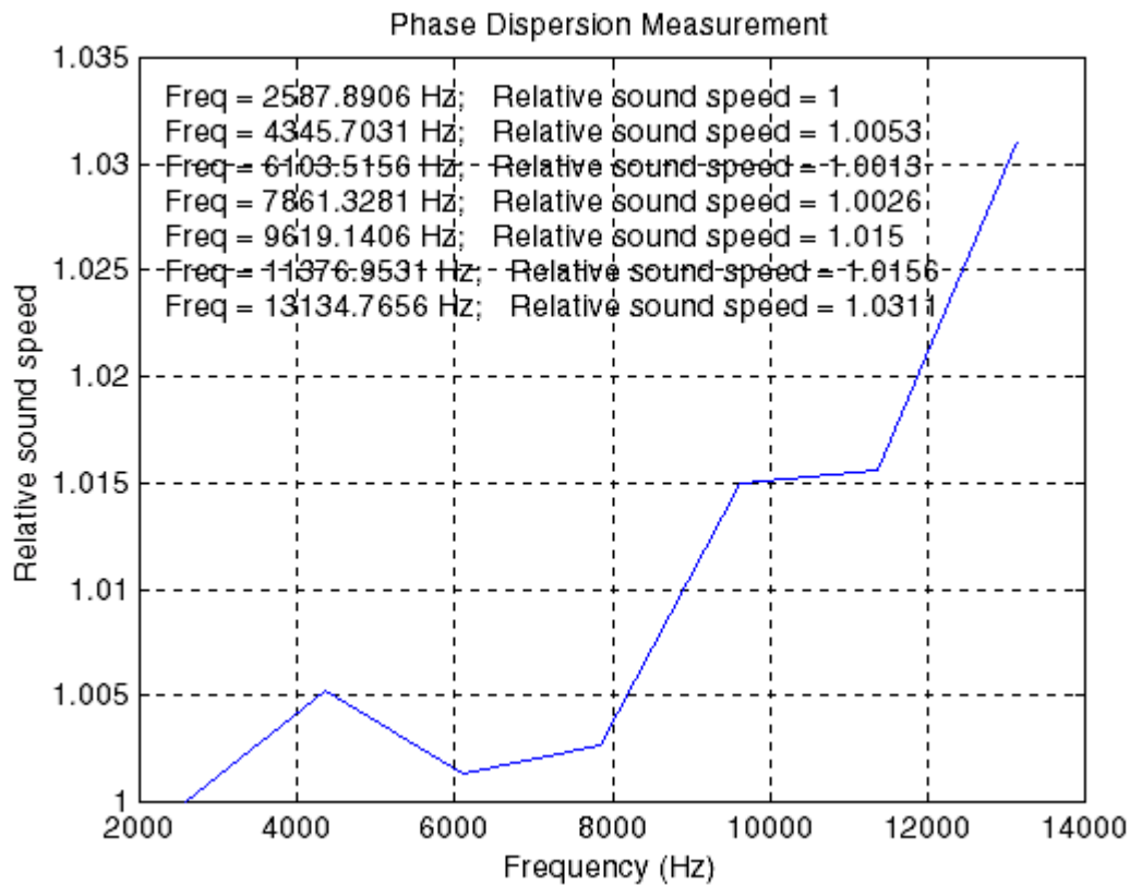
Figure 2. Relative sound speed as a function of frequency. The graph shows that sound speed increases by 3 % as frequency increases from 2.6 to 13.1 kHz.
