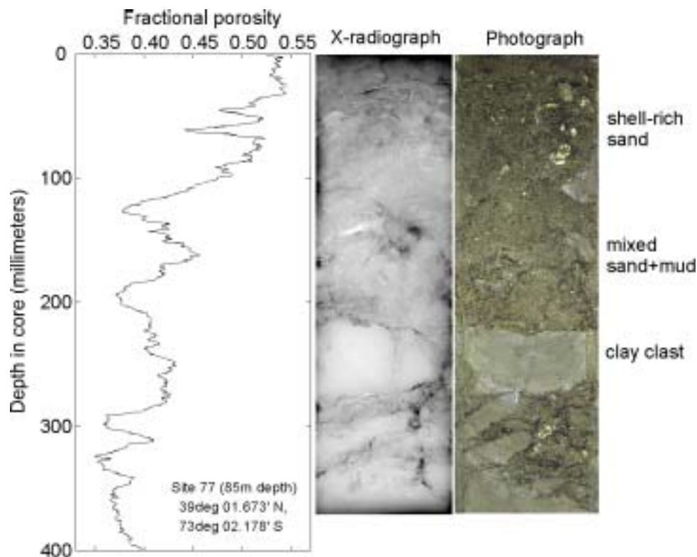
Figure 1. Example porosity profile, X-radiograph negative, and photograph of hydraulically damped core from the GeoClutter study site. A net downcore decrease in porosity is observed, as well as variability due to sediment grain size and consolidation state. Presence of mud clasts is indicative intense seafloor reworking at this depositional site.
