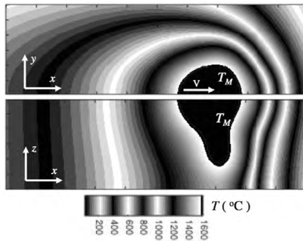
Fig. 28 Two-dimensional slices, at half workpiece top surface and longitudinal cross section at symmetry plane, of three-dimensional temperature field ( ^{\circ}\text{C} ) calculated using cross section information given in Table 1 for solidification boundary (WELD 9).
