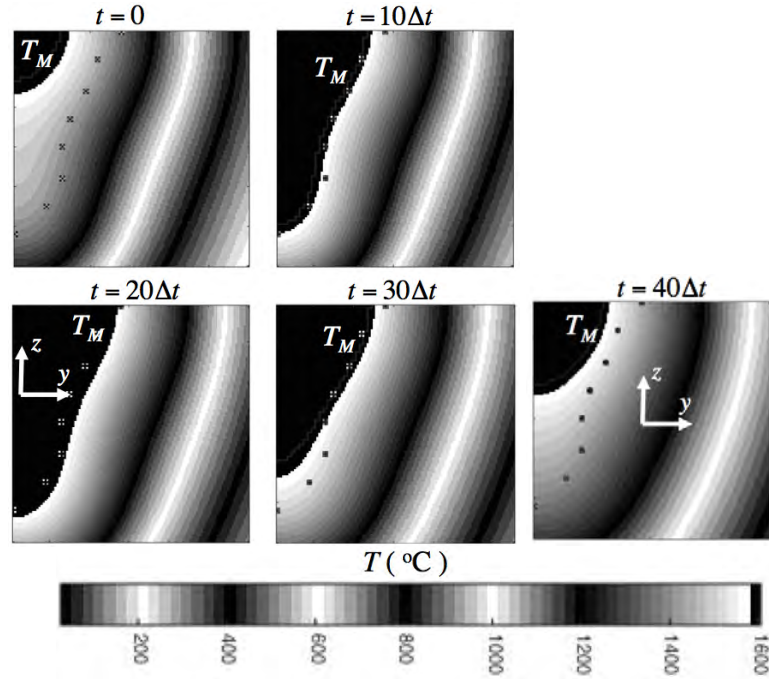
Fig. 9 Temperature history (°C) of transverse cross section of weld calculated using cross section information given in Table 1 for solidification boundary, where \Delta t = \Delta l / V , \Delta l = (1.512/60) mm and V = 5.0 mm/s (WELD 3).
