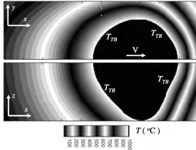
Fig. 10 Two-dimensional slices, at half workpiece top surface and longitudinal cross section at symmetry plane, of three-dimensional temperature field (°C) calculated using cross section information given in Table 1 for transformation boundary (WELD 3).
