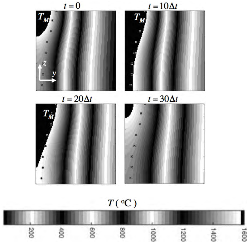
Fig. 19 Temperature history (°C) of transverse cross section of weld calculated using cross section information given in Table 1 for solidification boundary, where \Delta t = \Delta l / V , \Delta l = (3.0/60) mm and V = 5.0 mm/s (WELD 6).
