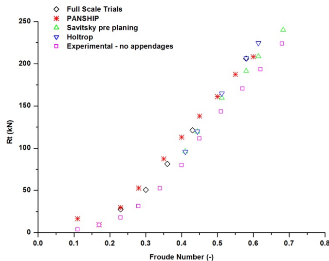
Figure 46 Sea Trial determined and Numerically predicted Total Resistance vs Froude Number (300 t displacement, 0.0 m static trim, trim tab in fully "retracted" position)
