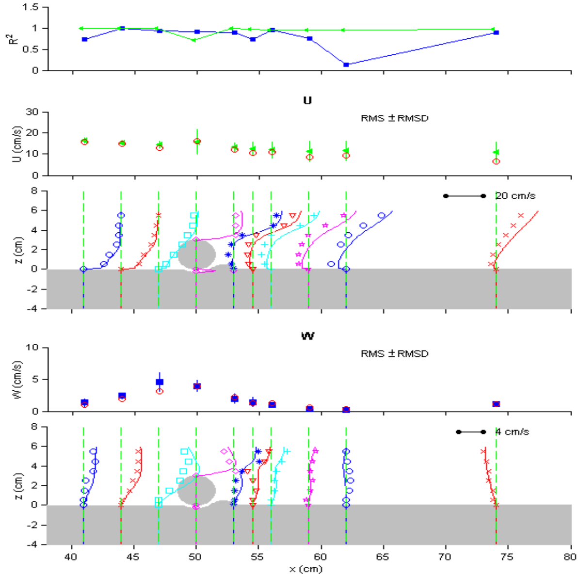
Figure 1. Model-Data comparisons of horizontal and vertical velocities Upper panel: model-data correlations for both horizontal, U , (triangles) and vertical, W , (squares) velocity. Second and Fourth Panel: Root-mean-squared values (RMS) and root-mean-squared deviations (RMSD) for U (triangles) and W (squares) respectively. The RMS of the laboratory data is represented by the circles. The RMSD values are shown by the error bars. Middle and bottom panel: Velocity profiles at different horizontal locations for U and W respectively. The symbols are the laboratory data and the solid lines are the model output. This figure shows scour profile 2, run with a variable 0.1 cm by 0.1 cm grid and the k - \epsilon turbulence model. Laboratory data obtained by B.L. Jensen et. al. (1990).
