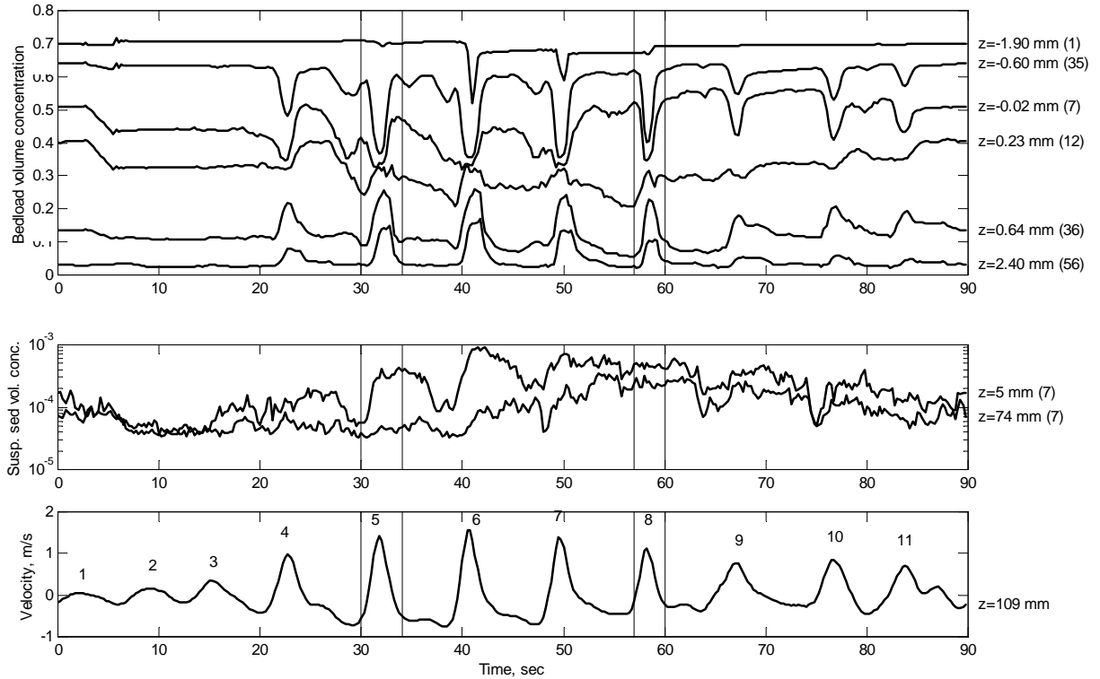
Figure 1: Sediment concentrations in the sheet flow layer (top panel) and in the suspension (middle panel) in relation to the near-bed orbital velocity (lower panel) under a wave group. These show bedload dilation down to -2\text{mm} in phase with the wave speed but no correlation between suspended concentration and instantaneous wave-current speed. Suspended concentration reaches a maximum of 10^{-3} (by volume) 5\text{mm} from the bed
