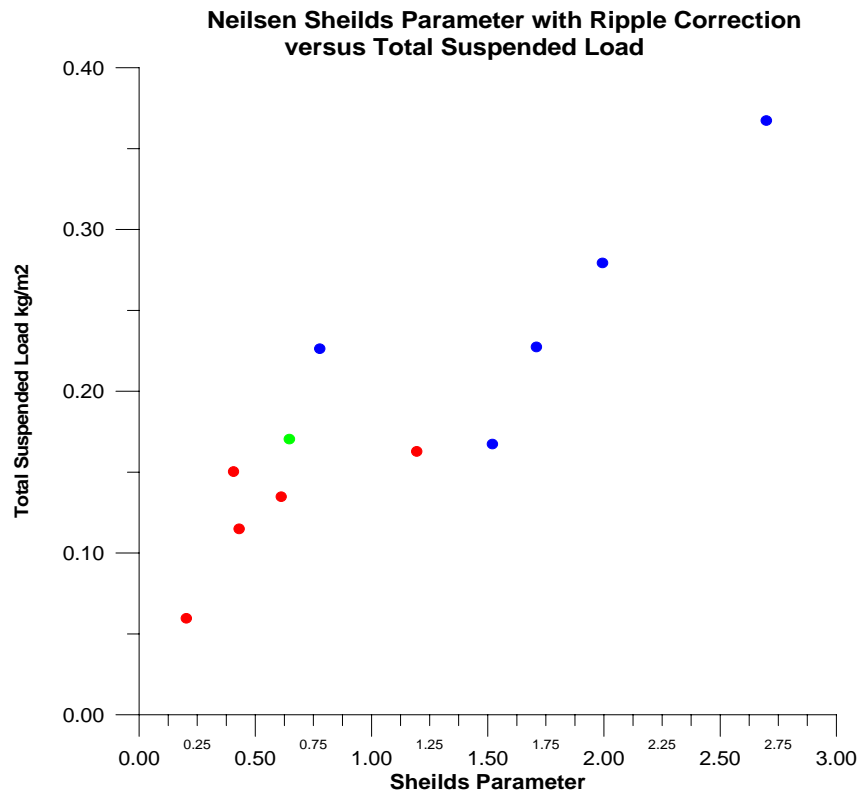
Figure 2: Total suspended load against the Nielsen Shields parameter with ripple correction. ● No infiltration, ● Half infiltration w_s=3.59 \times 10^{-4} \text{ ms}^{-1} , ● Maximum infiltration w_s=5.9 \times 10^{-4} \text{ ms}^{-1} . This shows that suspended load is decreased by a factor of two when percolation occurs through the sand bed
