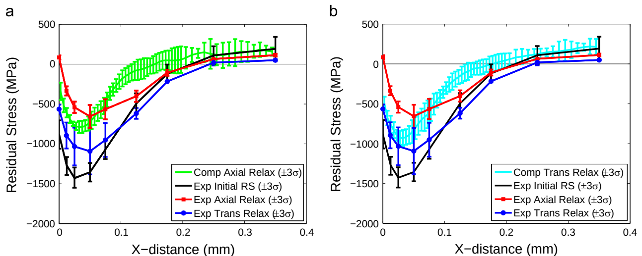
Fig. 11. Simulated versus experimental scatter in residual stress relaxation due to a single load/unload sequence for maximum applied stress \sigma_{\max} = 1050 MPa for N = 5 instantiations. The experimental residual stress scatter data are from Buchanan [45]. (a) Axial ( \sigma_{yy} ) relaxation, \sigma_{\max} = 1050 MPa, and (b) Transverse ( \sigma_{zz} ) relaxation, \sigma_{\max} = 1050 MPa.
