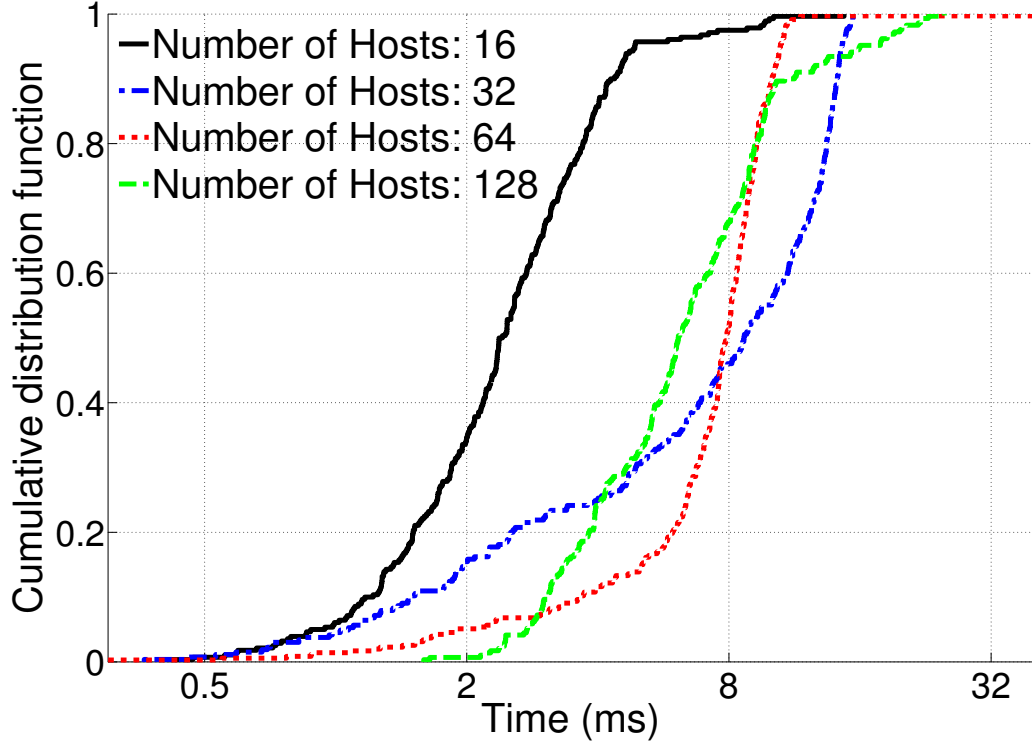
Figure 3.9: Buffering Delay of Merging Data from Hosts on Controller
