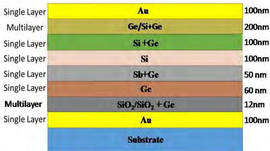
Figure 1: Cross-section of geometry used for typical multilayer thin-film system showing combination of single layers and multilayers.
