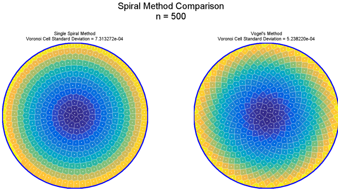
Fig. 25 Voronoi diagram comparison of single spiral and Vogel’s method for generating evenly spaced points on a disc
