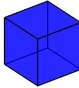
Hexahedron (Cube) 6 faces
