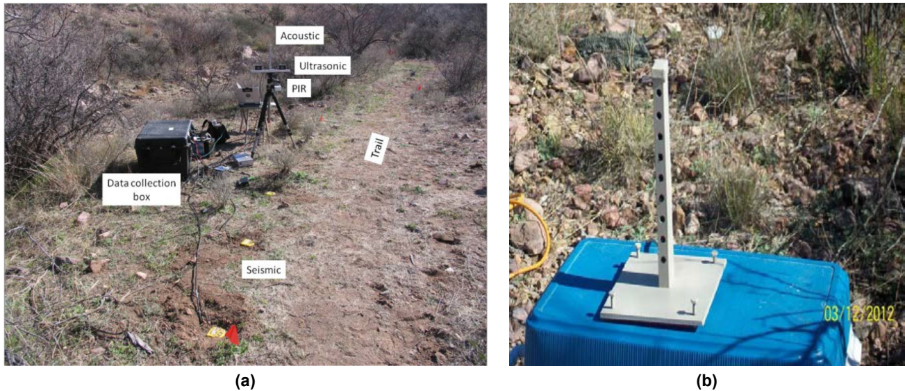
Figure 3: (a) ARL Sensor Deployment; (b) New Profiling Sensor.
