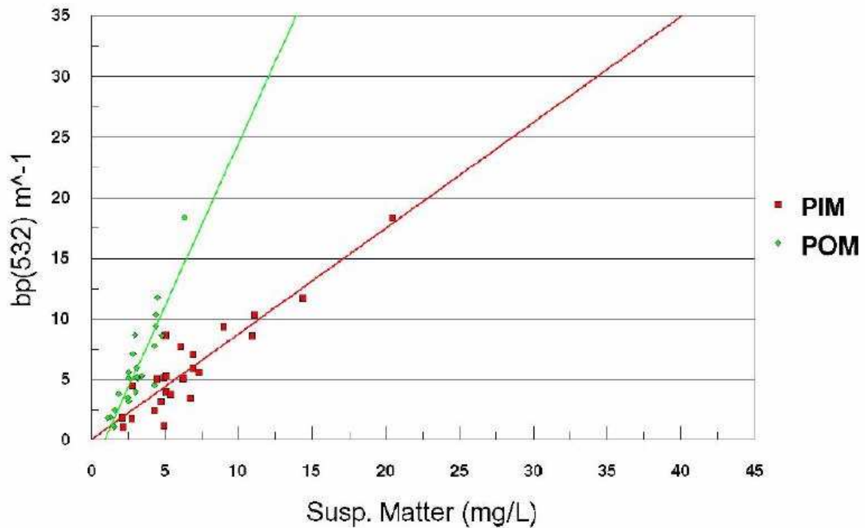
Figure 1. Regressions of mass of PIM and POM on particle scattering coefficient at 532 nm. PIM is not well correlated with the particle scattering coefficient, Mobile Bay, Alabama, May 2002.
