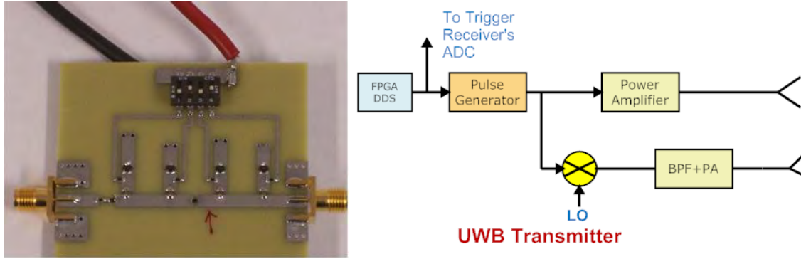
Figure 11 Stripline pulse generator and simplified mixer diagram for shaped UWB source
