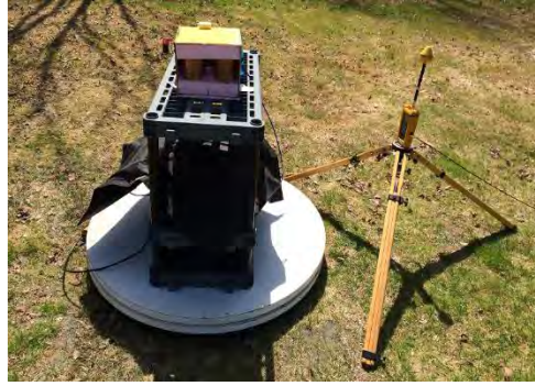
Figure 28 Radiation pattern measurement setup
