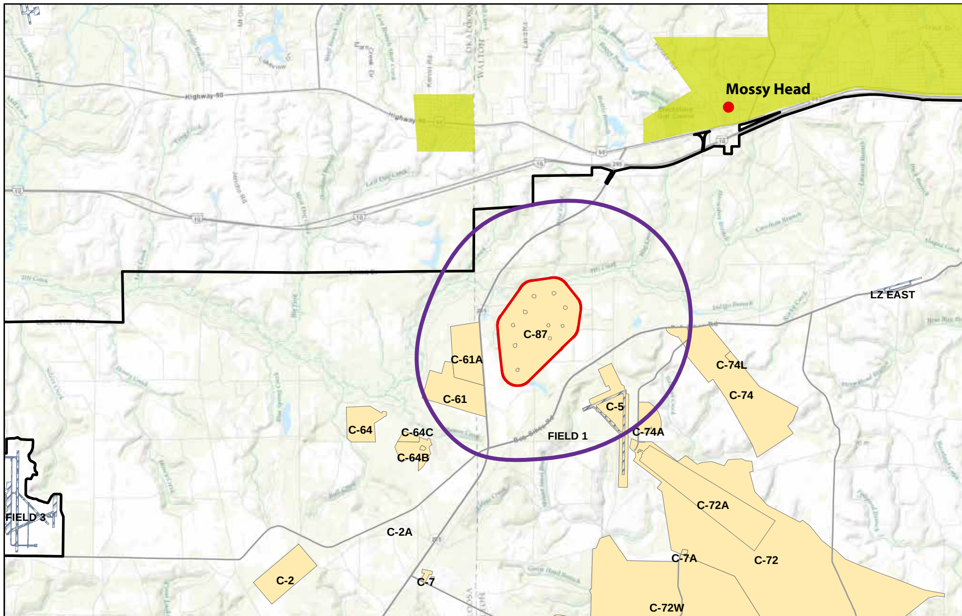
FIGURE 3-1 115 dB Noise Contour for 2.5 lb NEW Detonations at All Practical Training Sites on Test Area C-87 Under Favorable Weather Conditions Test Areas C-87 and D-51 REA
