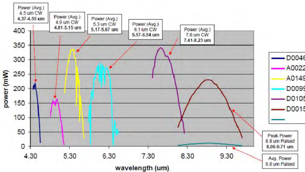
Figure 27. QCL wavelengths available for use in the AFIT CASI®.
