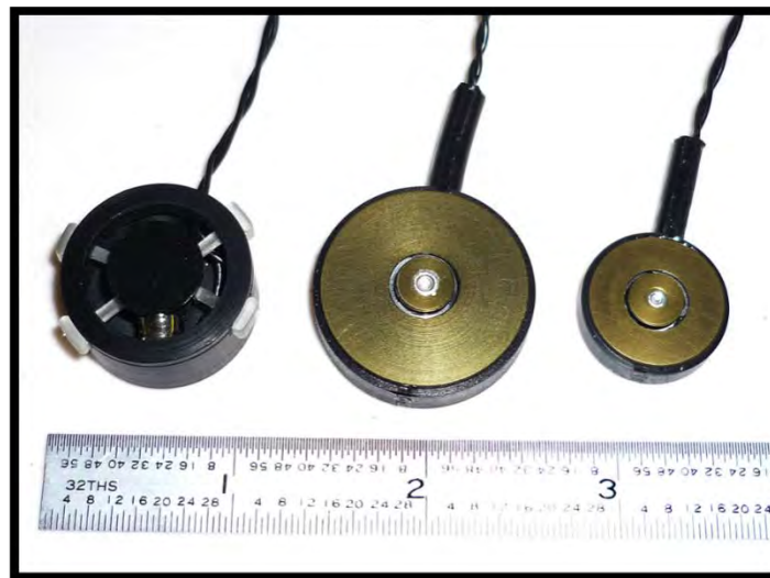
Fig. 2 EAI EMR, C-2, and C-3 tactor transducers (left to right)
