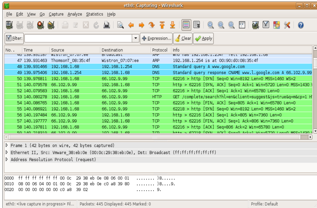
Figure 22: Wireshark Example
