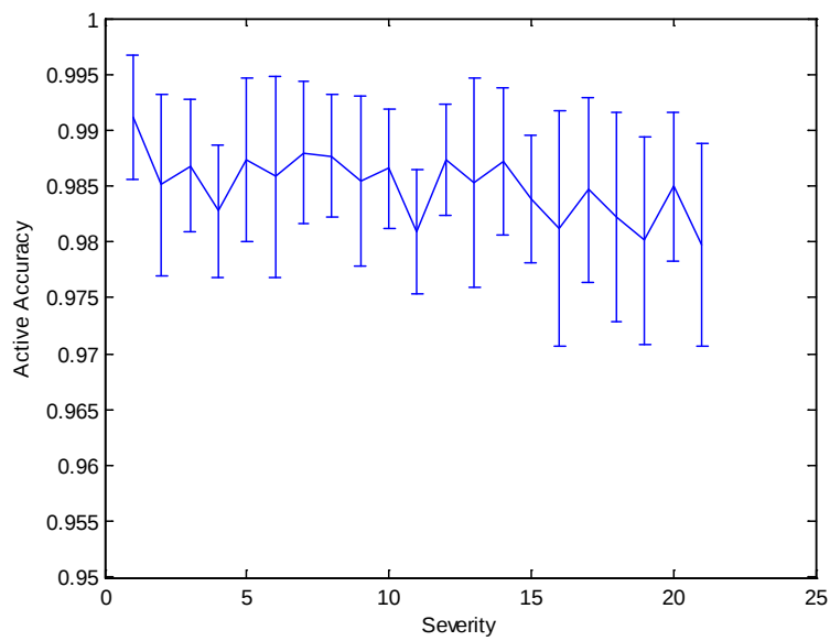
Figure 8: Active Accuracy Across Severity Levels
