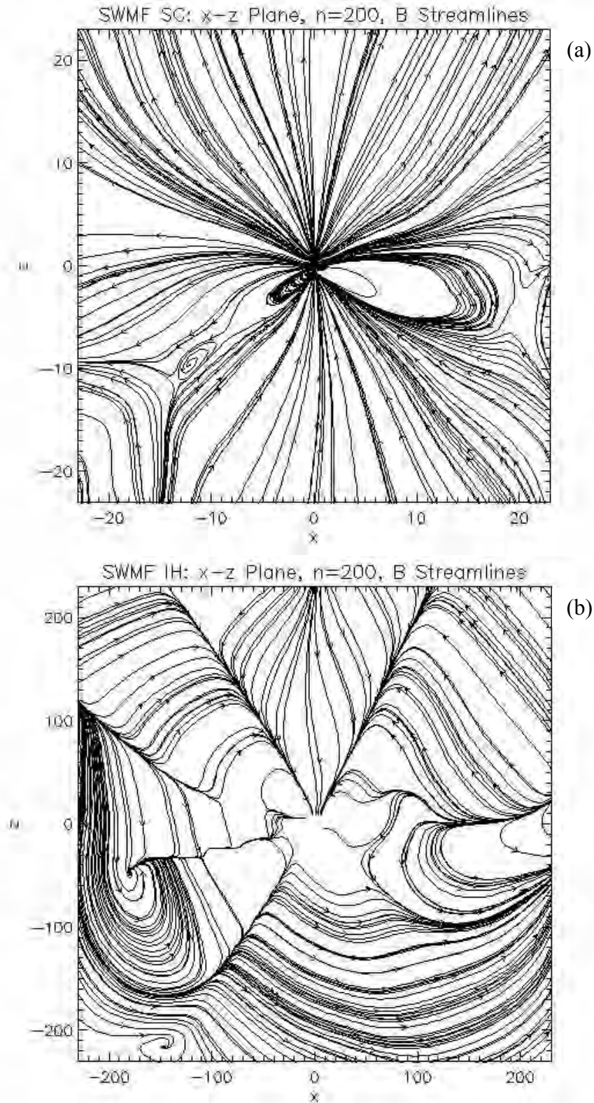
Figure 8. Streamlines of Magnetic Field on the x - z Plane for the n =200 Steady-State Solution for SC (a) and IH (b)
