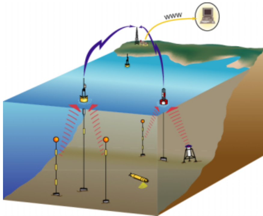
Figure 1. Concept drawing of the Portable Coastal Observatory illustrating the acoustic and RF data links from sea to shore and the final connection to the Internet.
