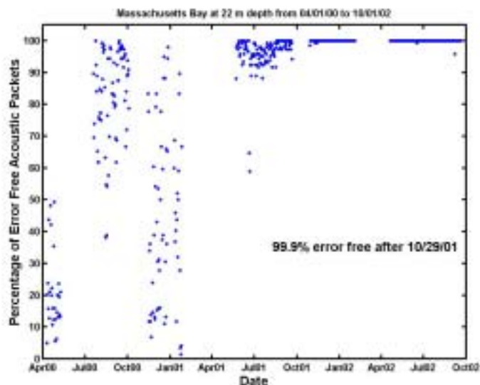
Figure 2. Acoustic error rates observed over 2 ½ years at the Scituate site in Mass Bay
