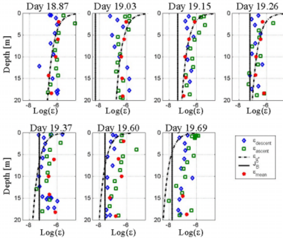
Figure 9. Variation in vertical distribution of rate of dissipation of kinetic energy observed during decent and ascent of the AUV during the passage of the atmospheric front
