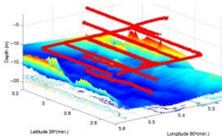
Figure 1 (a) OEX AUV and sensor systems, (b) AUV survey path
