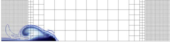
Figure 4: Static mesh for the density current case. The mesh is refined near the vertical edges of the domain to a 5^{th} level mesh (32 elements in the vertical direction, which corresponds to the resolution of the reference simulation). The middle of the domain is kept at 2^{nd} level mesh (coarsened three times to 4 elements in the vertical dimension). The results for 10^{th} order polynomials are obtained on the mesh one level coarser for both refined and coarse regions to keep the effective resolution comparable between 5^{th} and 10^{th} order. The color contours show the potential temperature perturbation.
