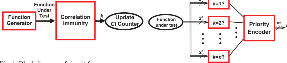
Fig. 1. Block diagram of circuit for computing correlation immunity.
