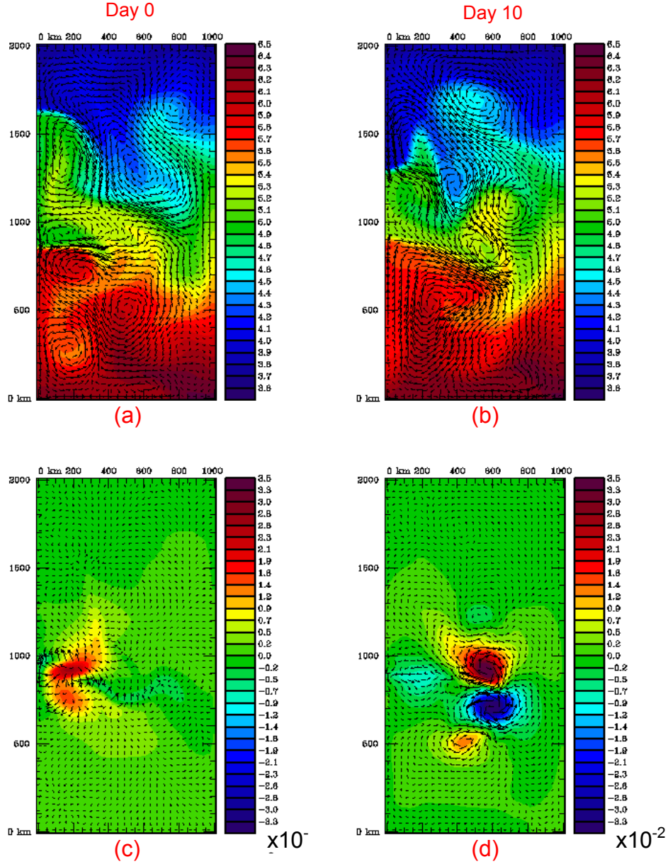
Figure 1: Panels a and b show the surface temperature and velocity vectors of the double gyre basic state flow 10 days apart. Panels c and d show the surface velocity and sea level at initial and final times for the optimal perturbation that maximizes the growth of perturbation energy over the 10 day period.
