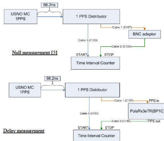
Figure 3.2 BIPM BP1C PPS IN/OUT measurements
