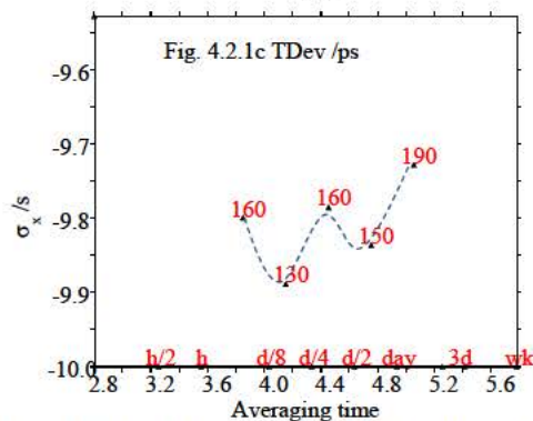
Figure 4.2.1 DCD of Lab(k)-PTB link comparison. Both TW and PPP links are calibrated
