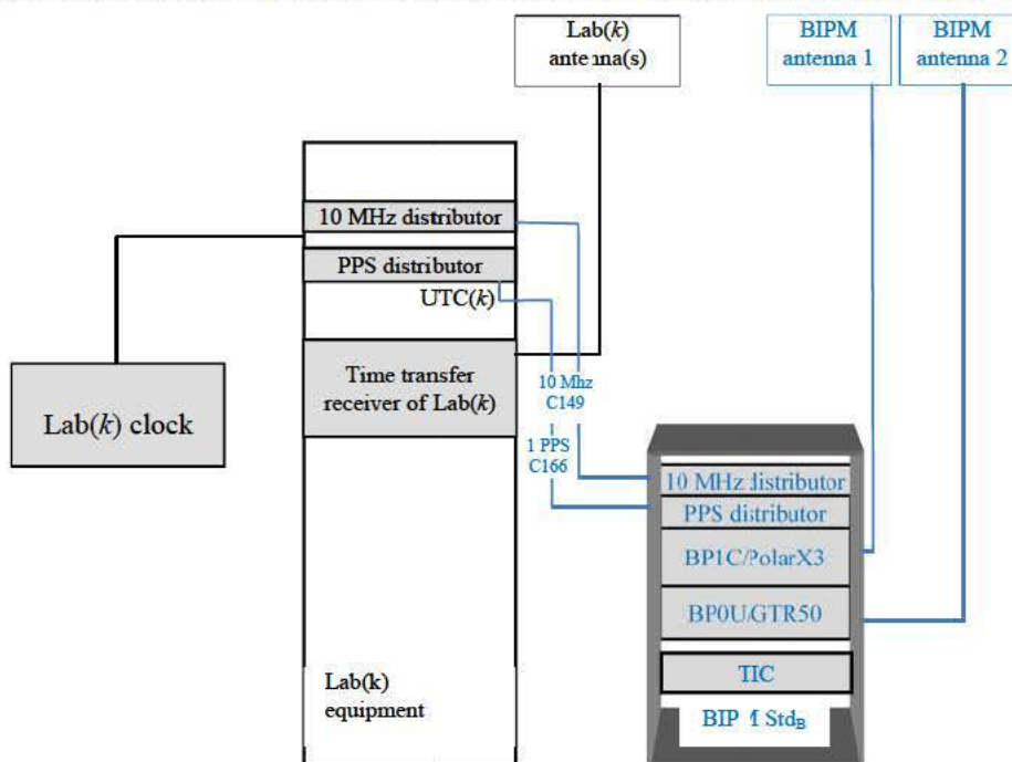
Figure 2 Setup of the BIPM Std_B at a UTC ( k )
