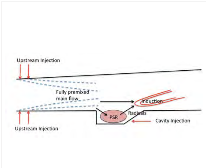
Figure 30: A conceptual model showing the cavity reaction represented by PSR model and the mixture of main and cavity reaction represented by a zero-dimensional ignition model.
