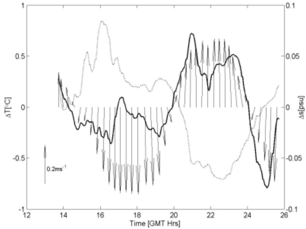
Figure 6. An overlay of current vector field at 9m depth, temperature variation, T , (thick line), and salinity variation, s , (dotted line) as determined from the AUV measurements. Each time series has been low-pass filtered at 15 minutes.
