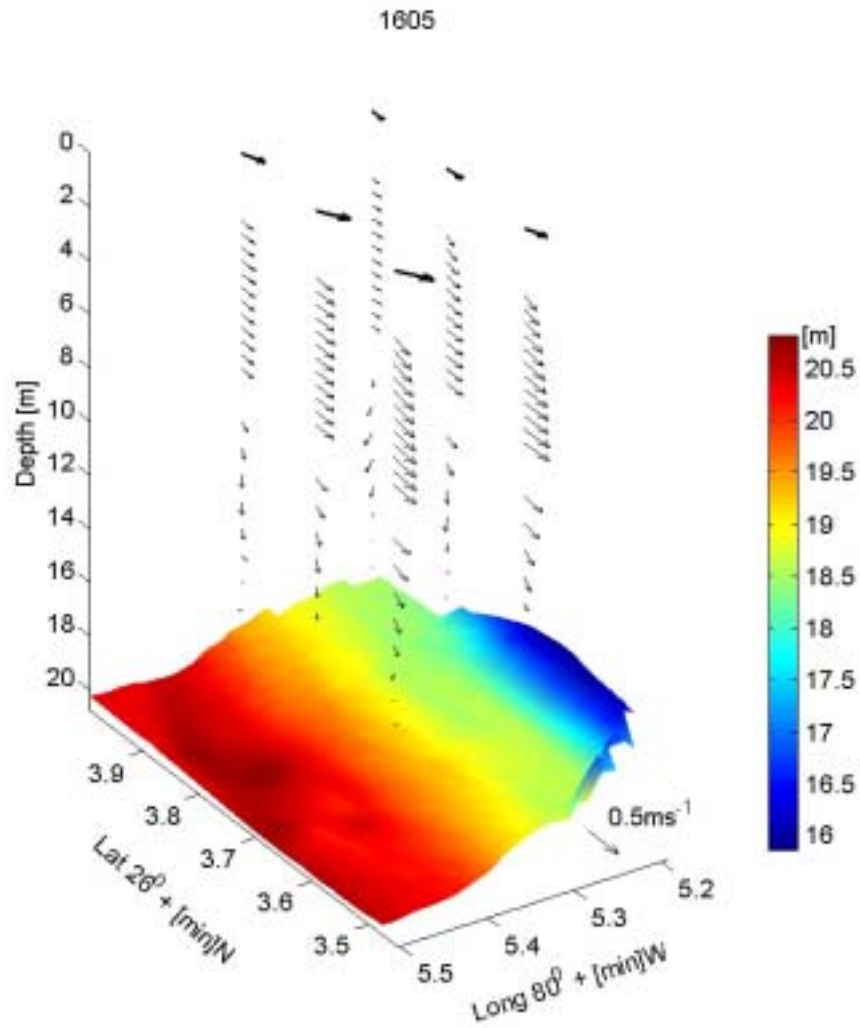
Figure 4 Current profile of the low-pass filtered (at 15 minutes) current-field at the six OSCR grid points as determined from the AUV survey during the second segment of the survey. The surface current vectors recorded by OSCR (thicker arrows) are overlaid. The colors indicate the local water depth
